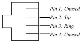
Connection pinouts
