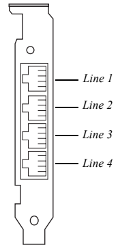
Voice board backplate
